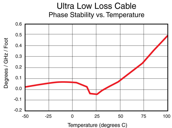
Fig. 6 – Plot of phase stability with temperature for several different test frequencies
